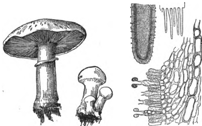
FIG. 327. — The common edible Mushroom, Agaricus campestris ; \times \frac{1}{2} . On the right, a section across several gills, \times 2 ; a section across one gill, \times 10 ; and a portion of one gill showing mycelium, hymenium, and basidia, with basidiospores, \times 25 . (From Bailey, and Sachs.)
